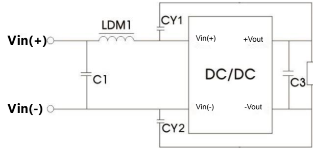
Figure 6-②. EMC Recommended Circuit
