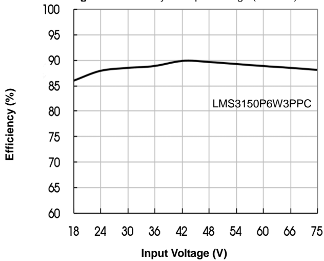
Figure 4. Efficiency vs. Input Voltage (full load)
