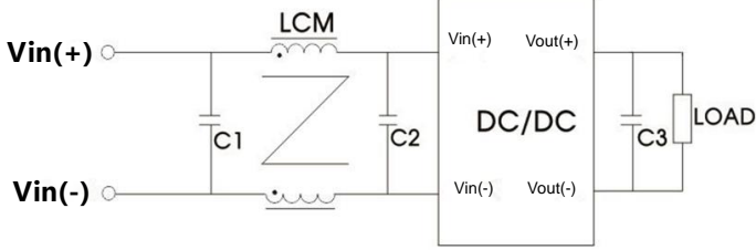
Figure 6-②. EMC Recommended Circuit
