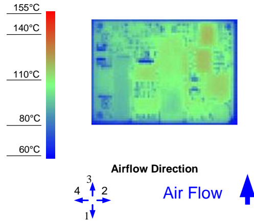
Figure 8. Thermal Image for Airflow Direction 3 (6.7A output, 55°C ambient, 200 LFM, typical Vin, open frame, unit soldered onto a fixture board)
