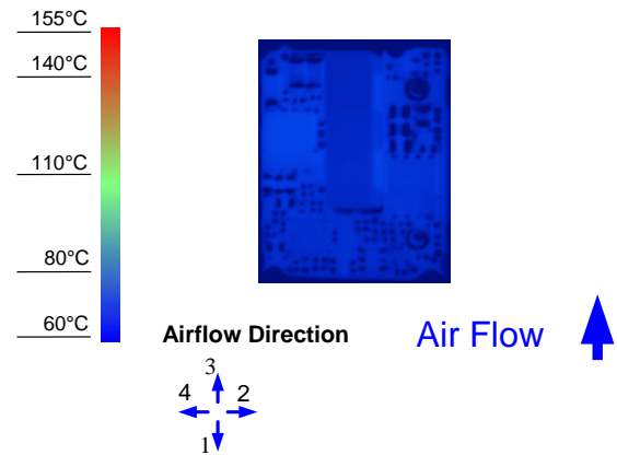
Figure 10. Thermal Image for Airflow Direction 3 (5A output, 55°C ambient, 200 LFM, typical V_{in} , open frame unit)
