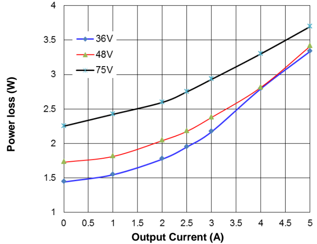
Figure 2. Power loss vs. Output Current (25°C)
