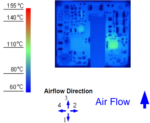
Figure 8. Thermal Image for Airflow Direction 3 (7A output, 55°C ambient, 200 LFM, typical Vin open frame unit, soldered interface)
