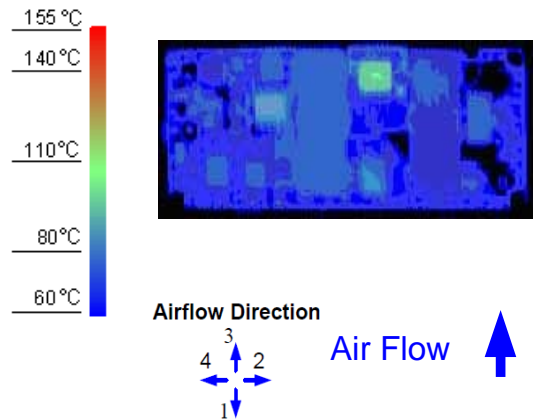
Figure 12. Thermal Image for Airflow Direction 3 (10A output, 55°C ambient, 200 LFM, typical V_{in} , open frame, socket interface)
