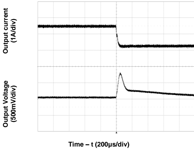
Time – t (200µs/div) Figure 7. Transient Load Response (typical Vin, load current steps from 50% to 25% at a slew rate 0.1A/µs)
