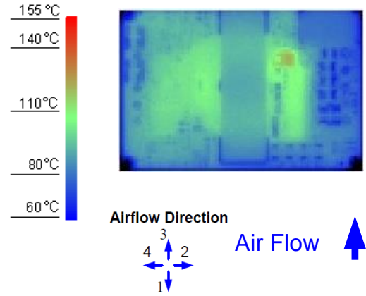
Figure 10. Thermal Image for Airflow Direction 3 (4.8A output, 55°C ambient, 200 LFM, typical Vin, open frame, soldered interface)
