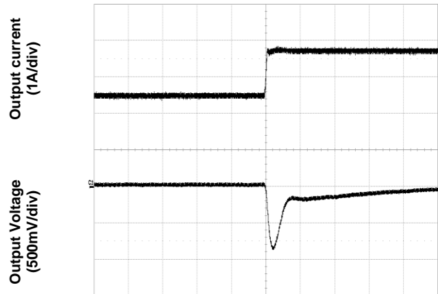
Time – t (200µs/div) Figure 8. Transient Load Response (typical Vin, load current steps from 50% to 75% at a slew rate 0.1A/µs)
