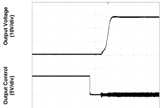
Figure 6. Start-Up from Enable Control (typical Vin and full load)
