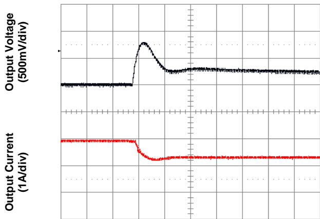
Figure 5. Transient Load Response (typical Vin, load current steps from 75% to 50% at a slew rate 0.1A/µs)
