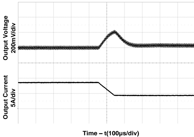
Figure 7. Transient Load Response (Typical V_{in} , load current steps from 50% to 25% at a slew rate 0.1A/\mu s )
