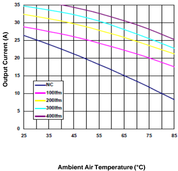
Figure 13. Current Derating Curve for Airflow Direction 2 (Ref. Figure 14 for Airflow Direction; Vin = 36V, open frame unit)
