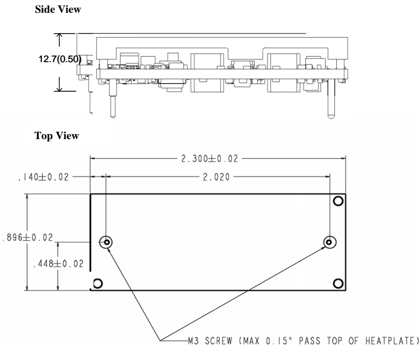
Figure 21. Converter with Open frame option
