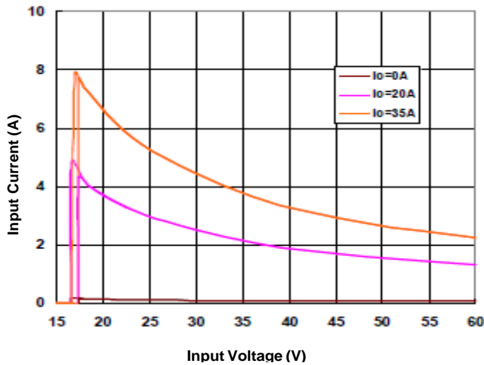
Figure 9. Input Characteristics
