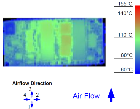
Figure 12. Thermal Image for Airflow Direction 3 (29.5A output, 55°C ambient, 200 LFM, typical Vin, open frame, socket interface)
