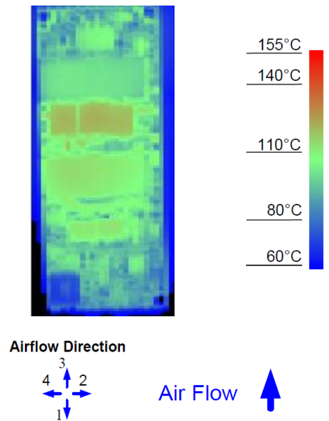
Figure 14. Thermal Image for Airflow Direction 2 (27.5A output, 55°C ambient, 200 LFM, typical Vin open frame, socket interface)
