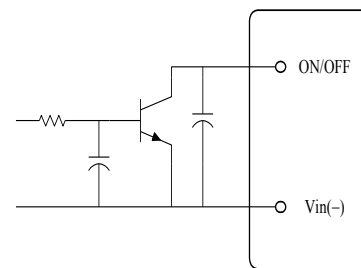
Figure. 16 Open Collector Enable Circuit
