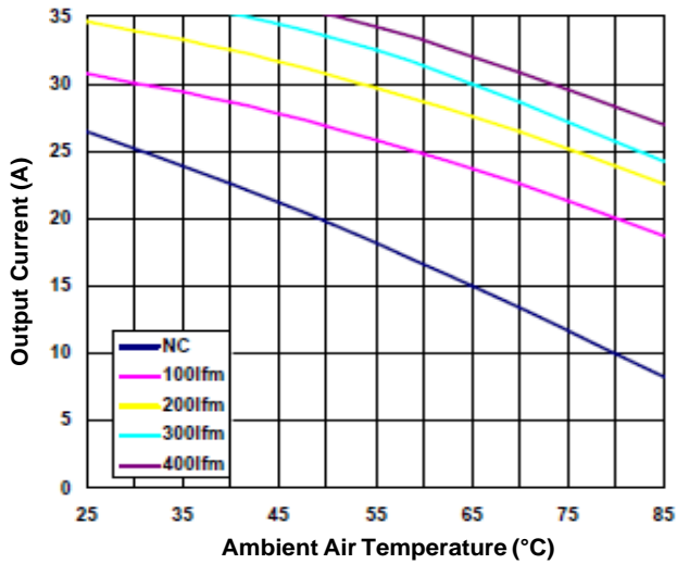
Figure 11. Current Derating Curve for Airflow Direction 3 (Ref. Figure 12 for Airflow Direction; Vin = 36V, open frame unit)
