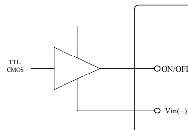
Figure. 17 Direct Logic Drive
