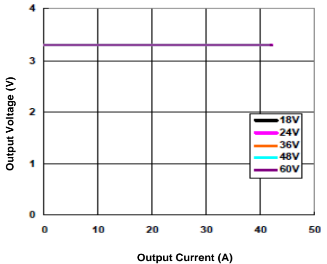
Figure 10. Output Characteristics
