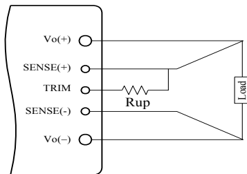
Figure. 19 Circuit to Increase Output Voltage
