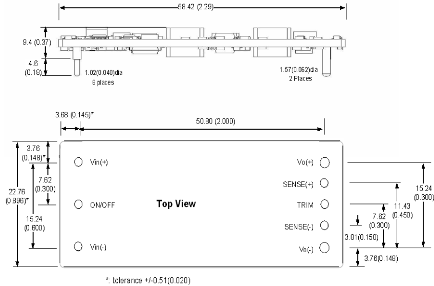
Figure 21. Converter with Open frame option
