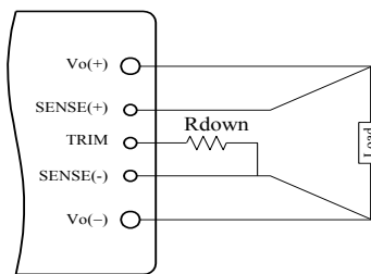
Figure. 18 Circuit to Decrease Output Voltage
