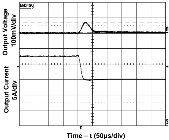
Figure 6. Transient Load Response
