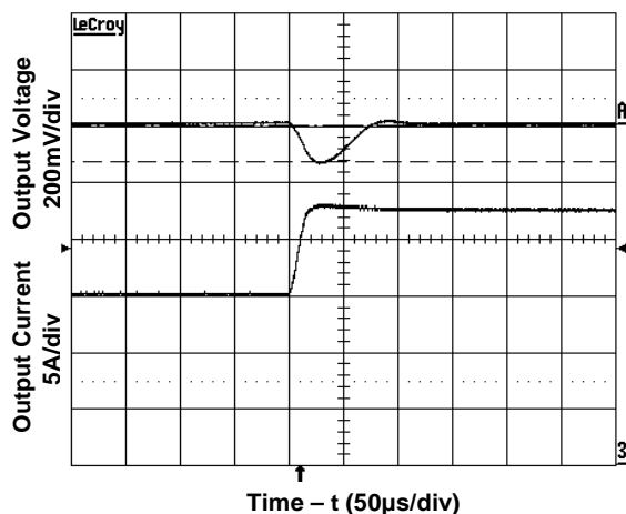
Figure 5. Transient Load Response
