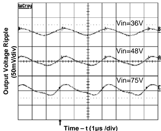
Figure 4. Output Ripple Voltage at Full Load
