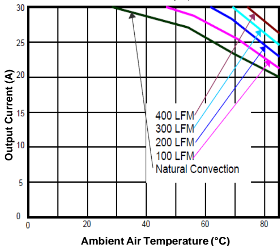
Figure 7. Current Derating Curve for Airflow Direction 3 (Ref. Figure 9 for Airflow Direction; Vin = 36V, open frame unit)
