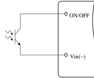
Figure 9. Opto Coupler Enable Circuit
