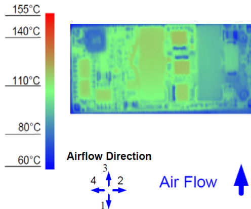
Figure 8. Thermal Image for Airflow Direction 3 (27.7A output, 70°C ambient, 200 LFM, typical Vin, open frame, socket interface)
