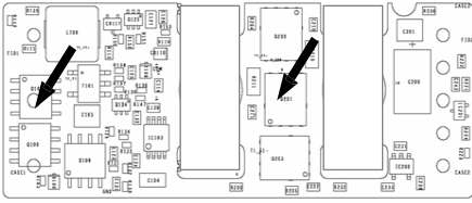
Figure 14. Temperature Monitoring Location
