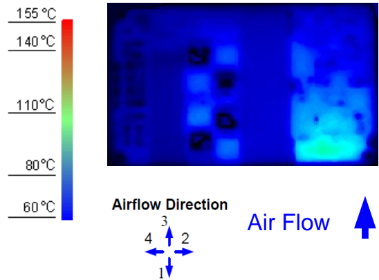
Figure 10. Thermal Image for Airflow Direction 3 (40A output, 55°C ambient, 200 LFM, typical Vin, open frame, soldered interface)
