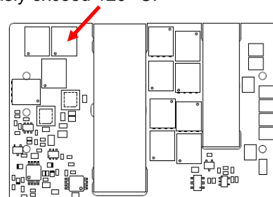
Figure 16. Temperature Monitoring Locations
